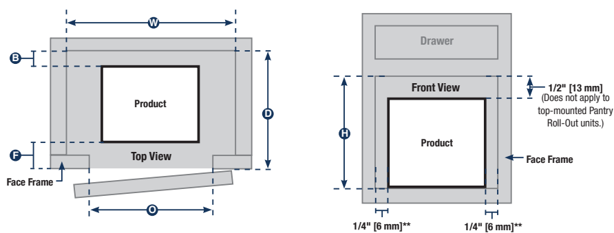
Example of Face Frame Cabinet Application
