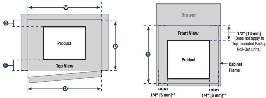
Example of Frameless / Euro-Style Cabinet Application
